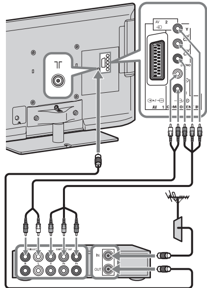
Audio/video device
